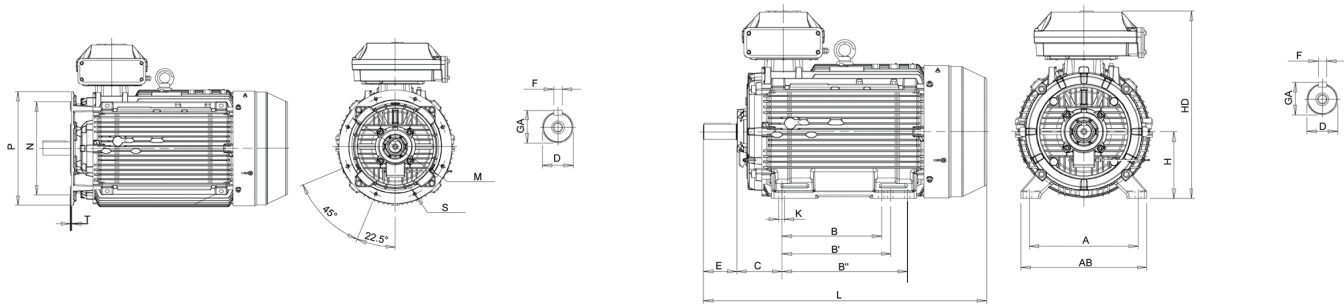
Foot-mounted motor IM1001, B3 and Flange-mounted motor IM 3001, B5
